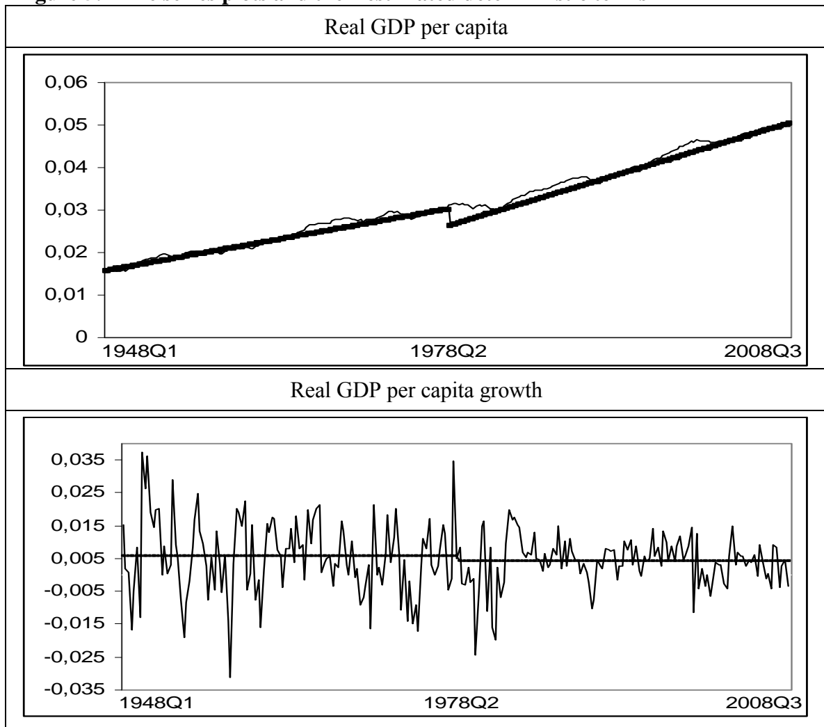
Figure 5: Time series plots and their estimated deterministic terms
