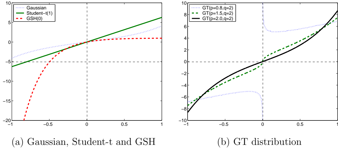
Figure 2: \phi -functions for different distributions
