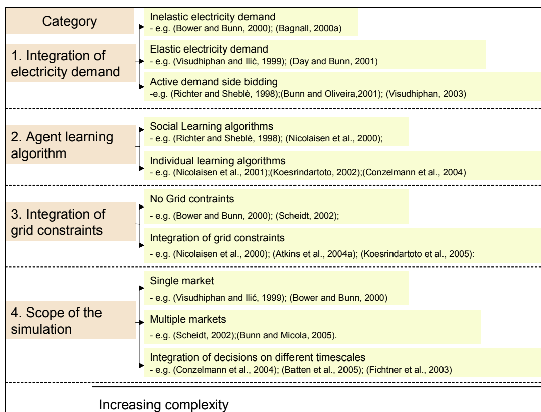
Figure 6: Examples for the increasing complexity of agent-based simulations
