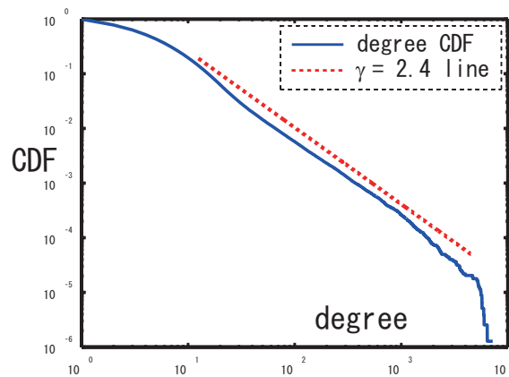
Figure 3: Degree distribution of Japanese firms' transaction network
