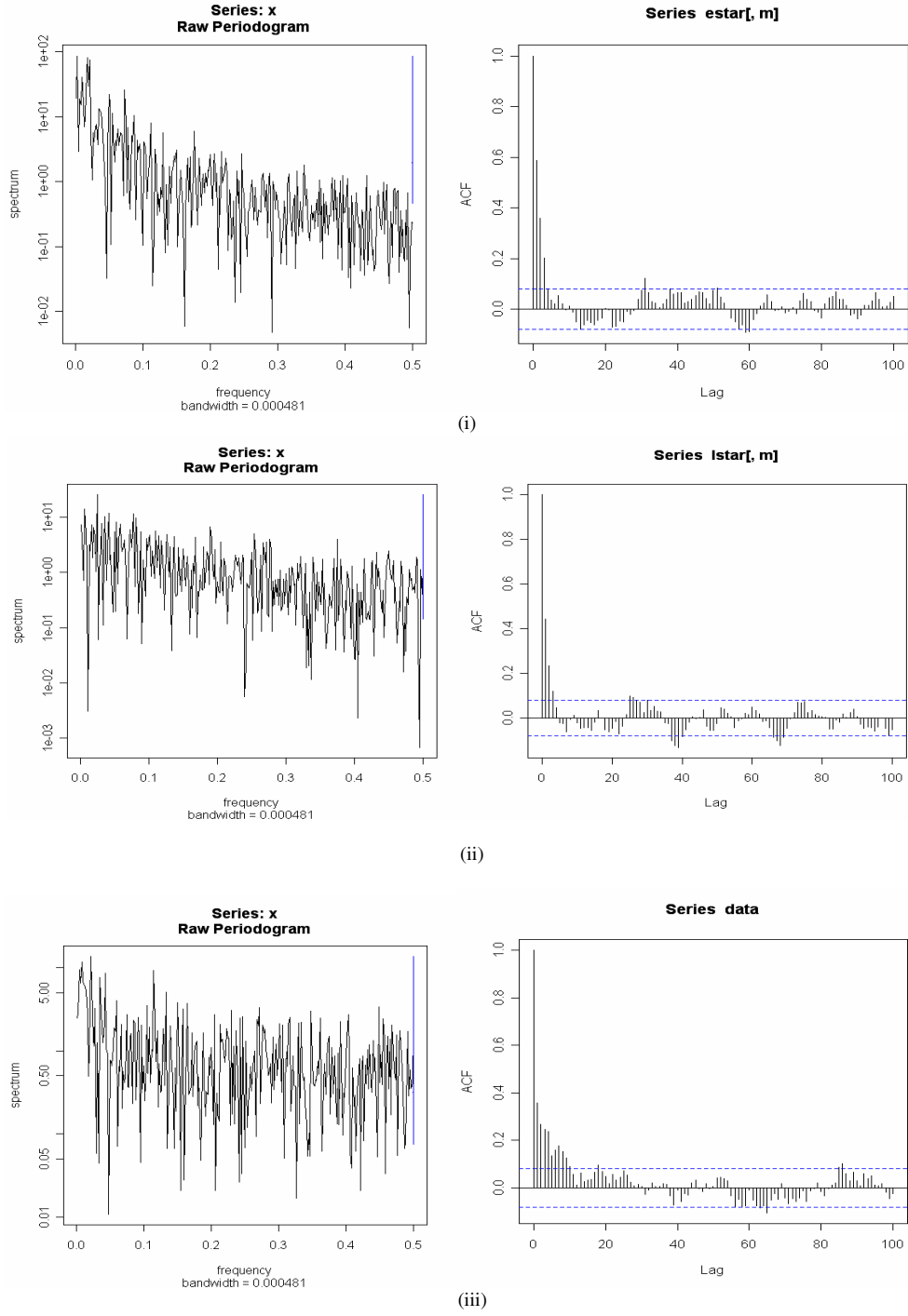
Figure 5: Sample periodograms and ACF plots (i) ESTAR process (ii) LSTAR process (iii) Long memory with d = 0.3427
