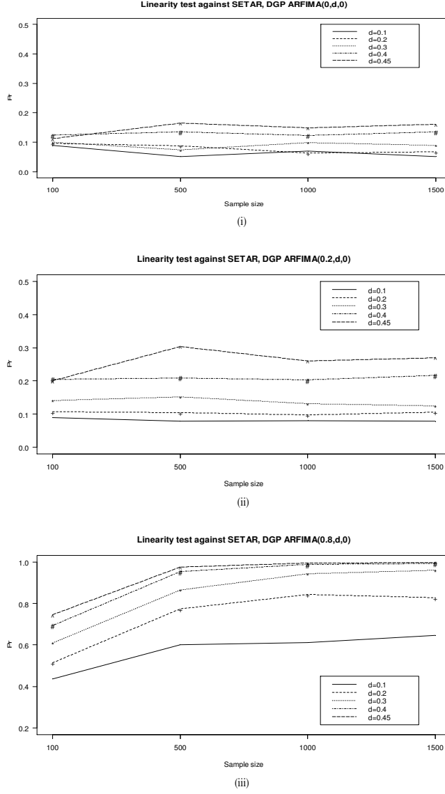
Figure 1: Rejection probabilities of linearity test against SETAR model (i) DGP is ARFIMA(0, d ,0),(ii) DGP is ARFIMA(0.2, d ,0) and (iii) DGP is ARFIMA(0.8, d ,0)
