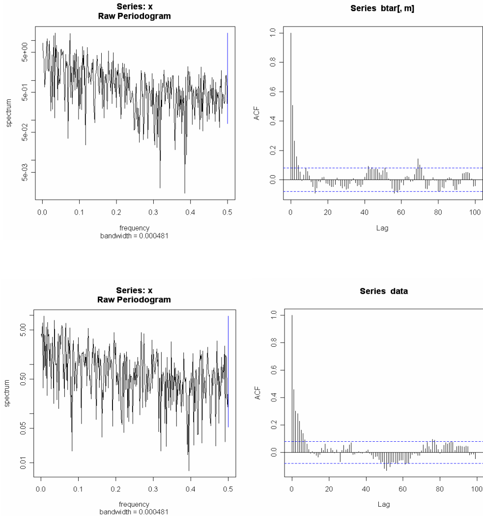
Figure 4: Sample periodograms and ACF plots (i) SETAR process (ii) Long memory with d = 0.3419
