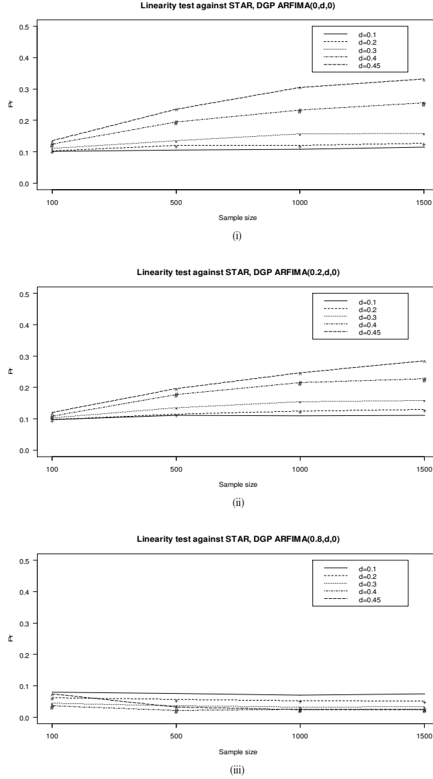
Figure 2: Rejection probabilities of linearity test against STAR model (i) DGP is ARFIMA(0, d ,0),(ii) DGP is ARFIMA(0.2, d ,0) and (iii) DGP is ARFIMA(0.8, d ,0)
