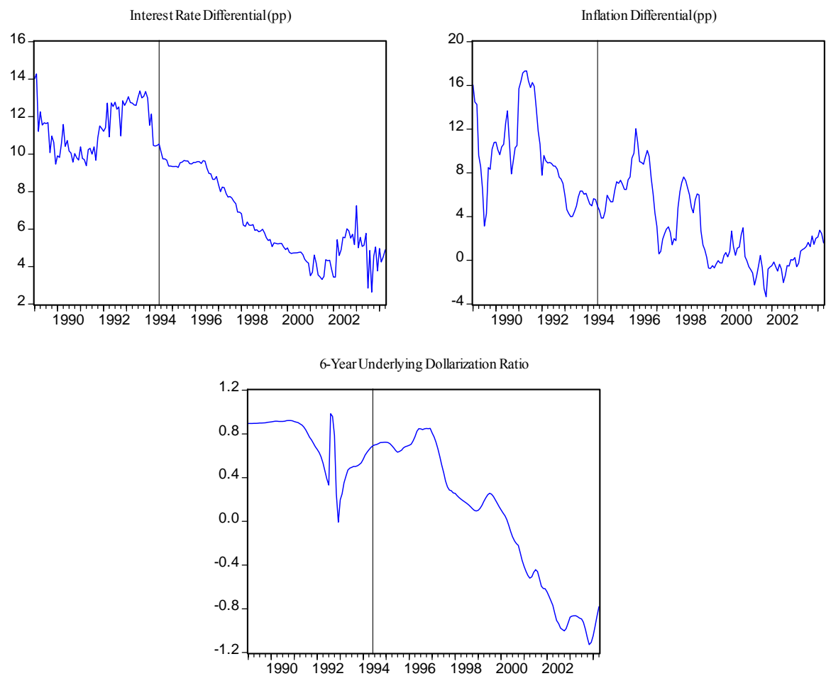
Figure 2. Explanatory Variables.
