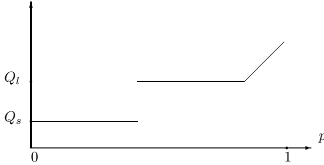
Figure 5. The figure depicts a provision rule with two bunching regions. For large p the provision rule is strictly increasing and coincides with the modified Samuelson Rule, Q^* .
