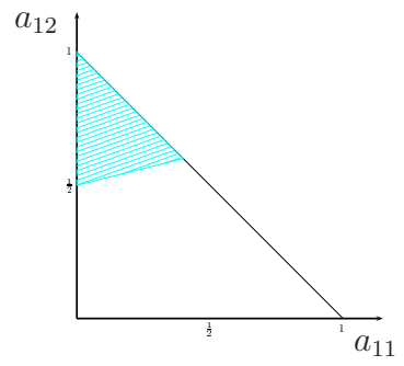
Feasible sets \mathcal{S}_6
