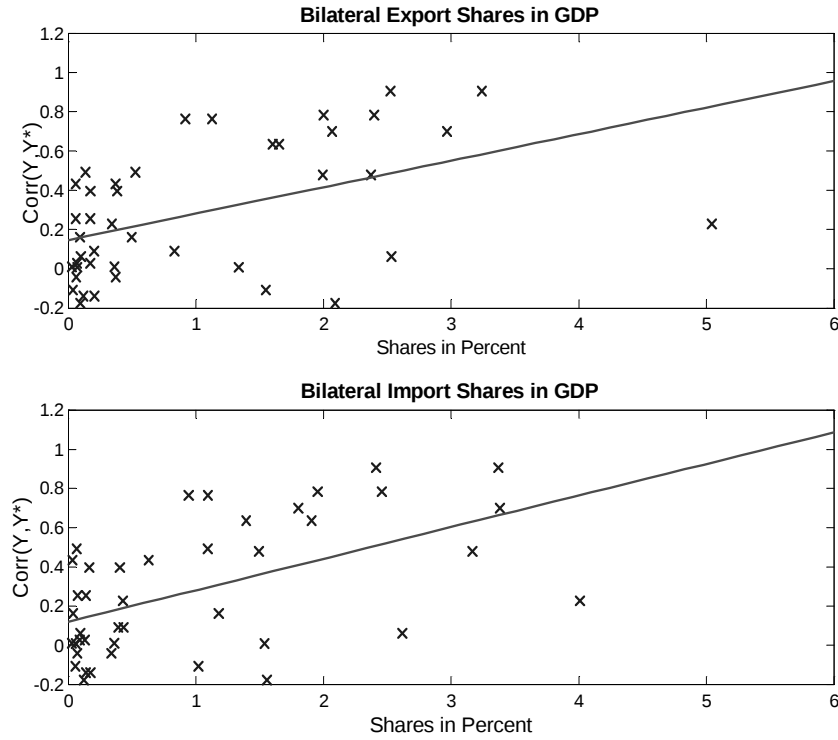
Figure 4.4: Trade Interdependence and Output Correlation amongst G7 Countries
