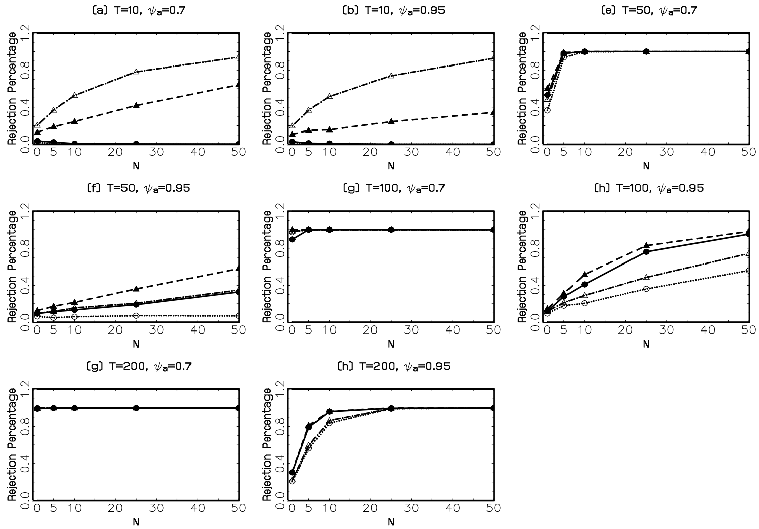
Figure 3: Empirical power results of the tests for DGP A and true cointegrating rank of two when hypothesized rank is one. ●——— panel SL-asympt, ▲ — — — panel SL-VAR(1), ○..... LLL-asympt, Δ - · - · - LLL-VAR(1).
