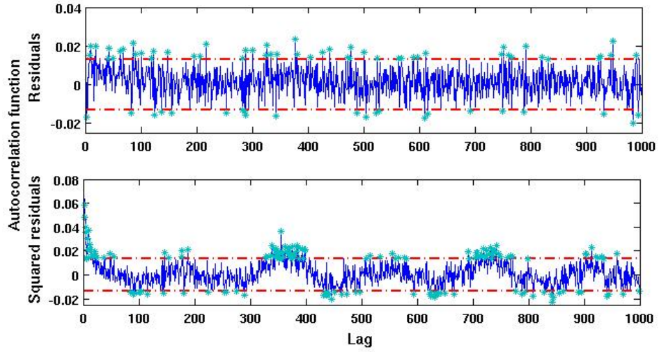
Figure 5: ACF for residuals \hat{\varepsilon}_t (up) and squared residuals \hat{\varepsilon}_t^2 (down) of the AR(3) during 19480101-20080527
