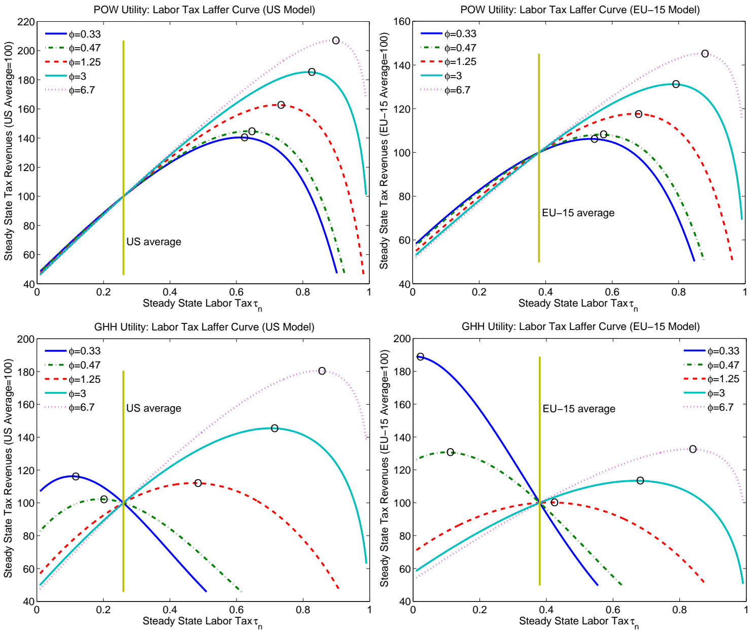
Figure 3: Sensitivity analysis on \phi' and \phi'' .
