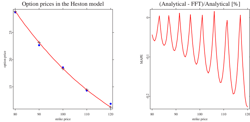
Figure 1.2: Left panel: European call option prices obtained by Monte Carlo simulations (filled circles), analytical formula (crosses) and the FFT method (solid line) for the Heston model. Right panel: Percentage differences between analytical and FFT prices.
