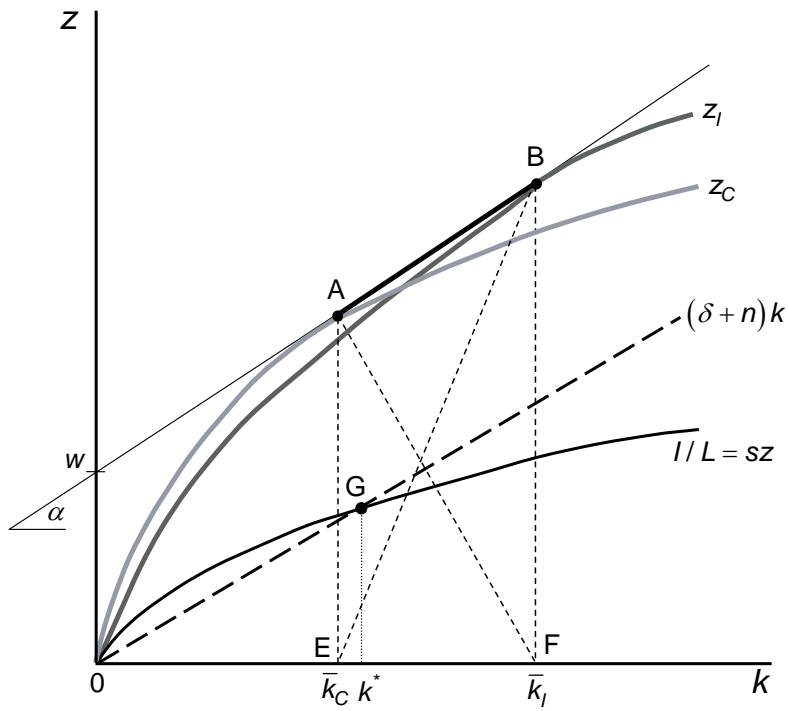
Figure 1. The Deardorff Diagram
