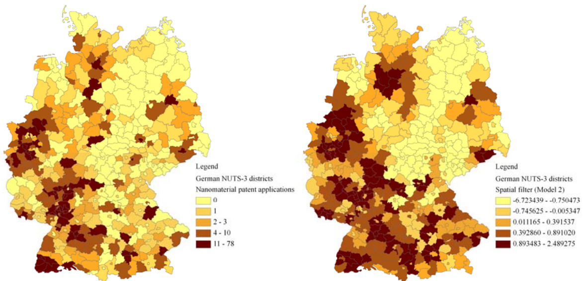
Figure 3: Comparison between the geographical distributions of nanomaterial patent applications (left) and of the spatial filter computed for Model 2 (right)
