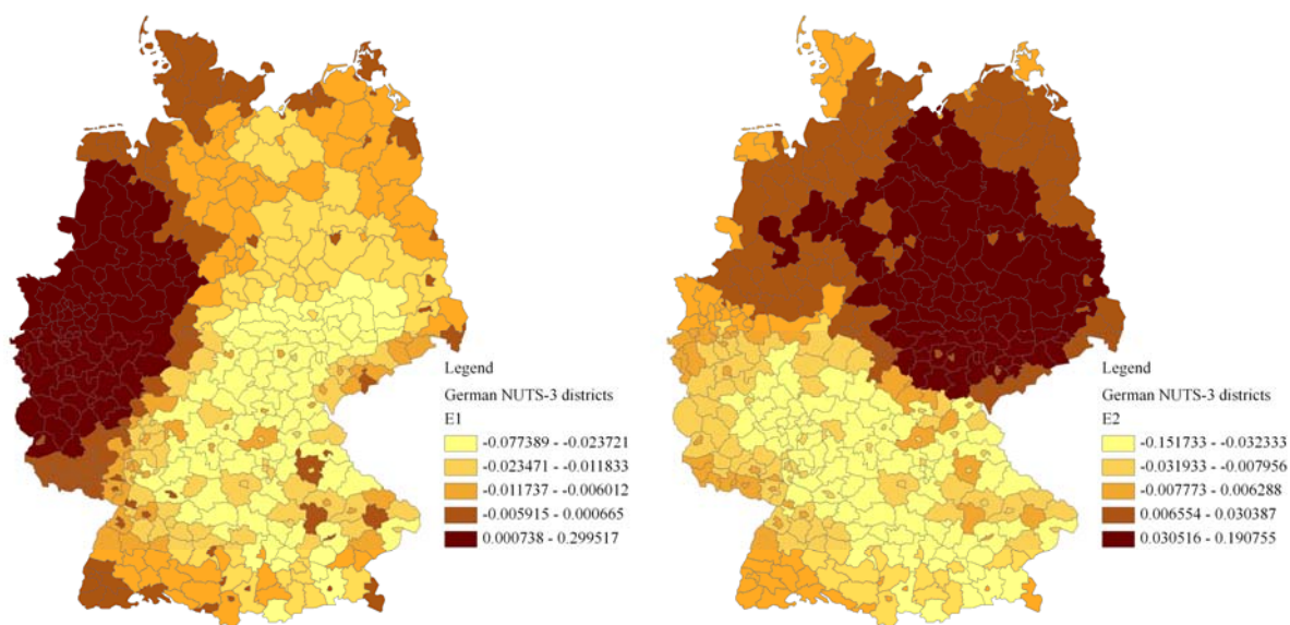
Figure 4: First two eigenvectors (E1, E2) extracted from the transformed spatial weights matrix W
