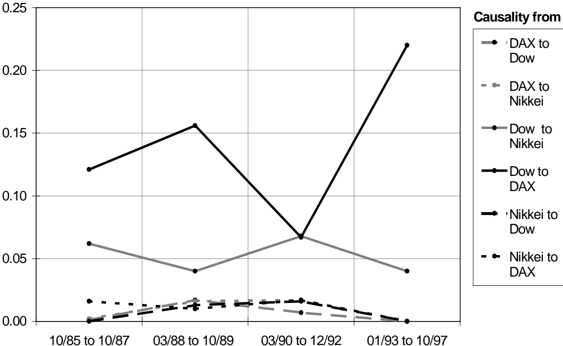
Figure 4-6: Hosoya's Measure for Causality from x to y
