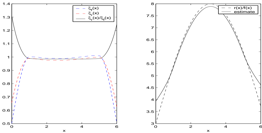
Figure 8: Proportionality of the bias: N = 2000 , y = 3 + 5\sin(0.5x) , x \sim U[0, 6] , h = 0.5 , \xi_f(x) and \xi_r(x) are means of 1000 samples
