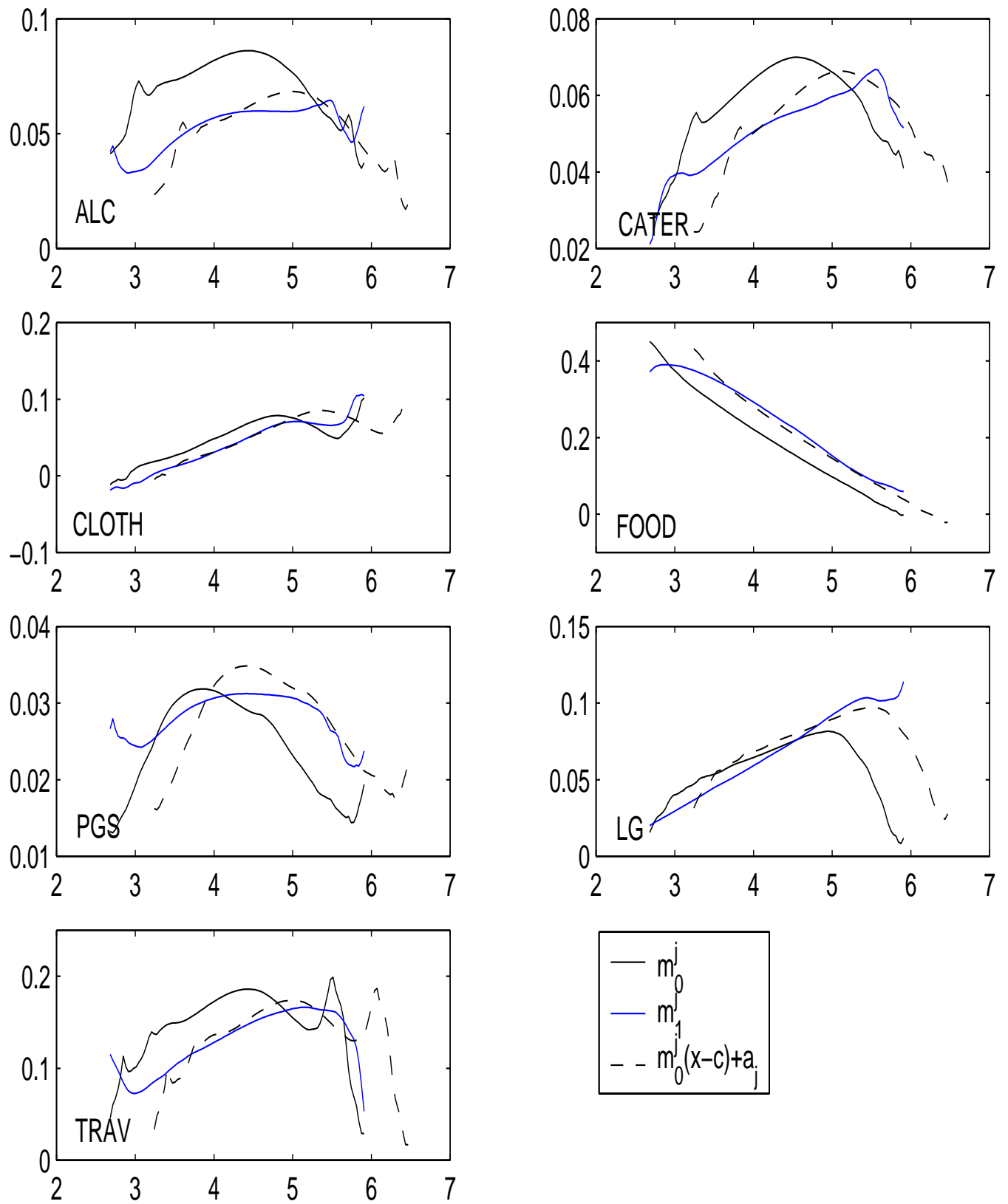
Figure 14: FES II, EPLM, variable bandwidth
