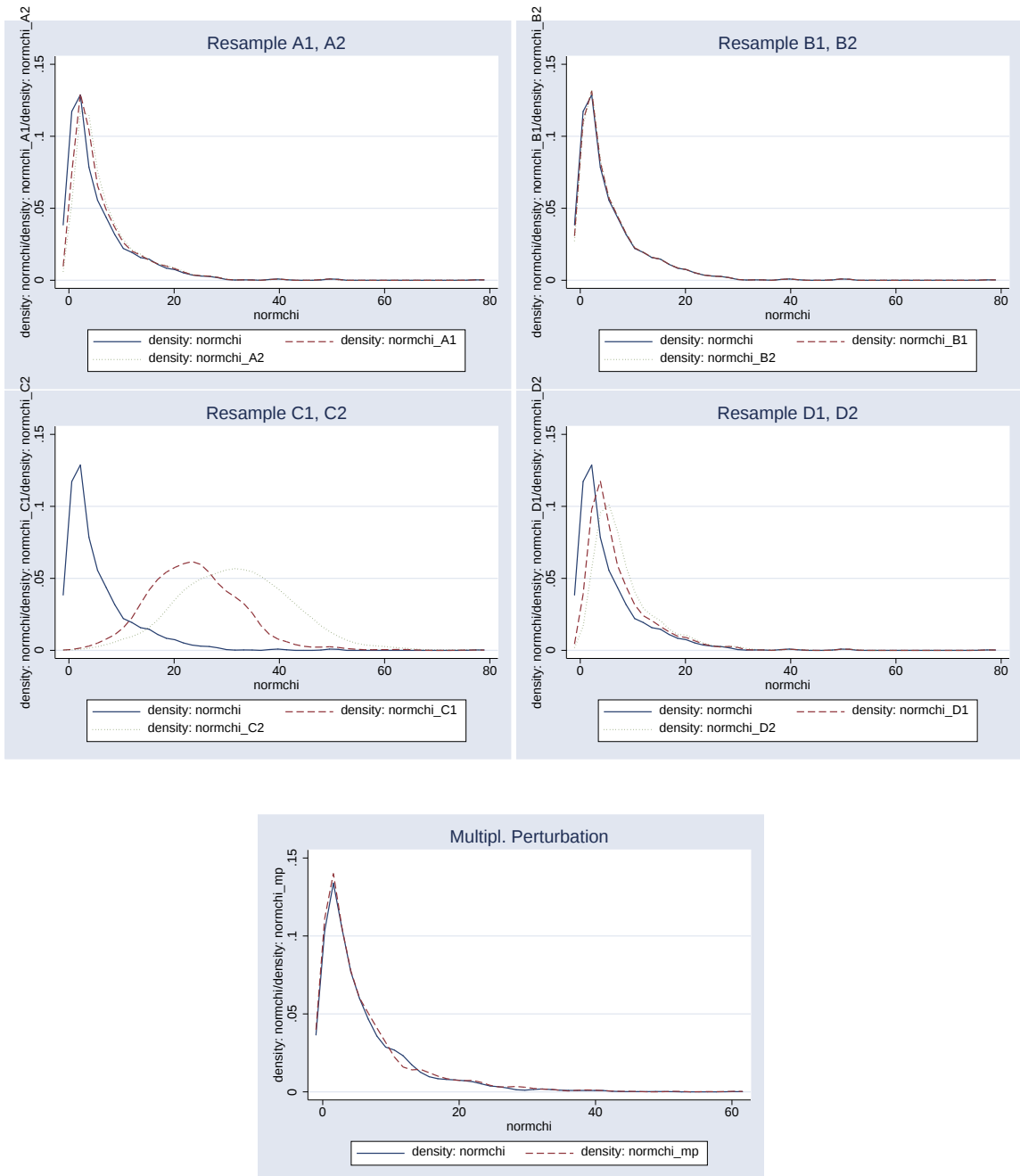
Figure 5: Mixed Distribution 1
