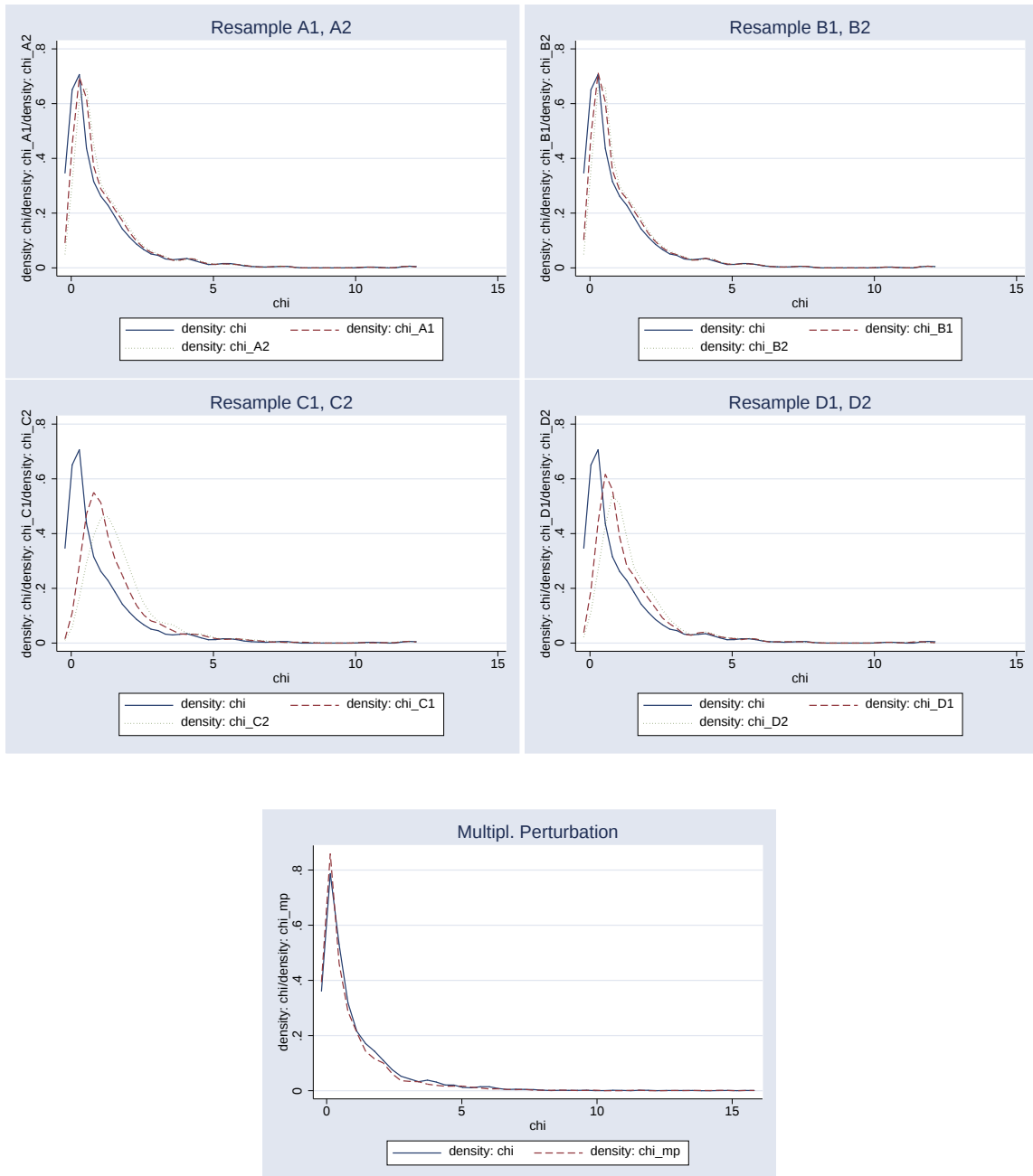
Figure 3: Chi-square Distribution
