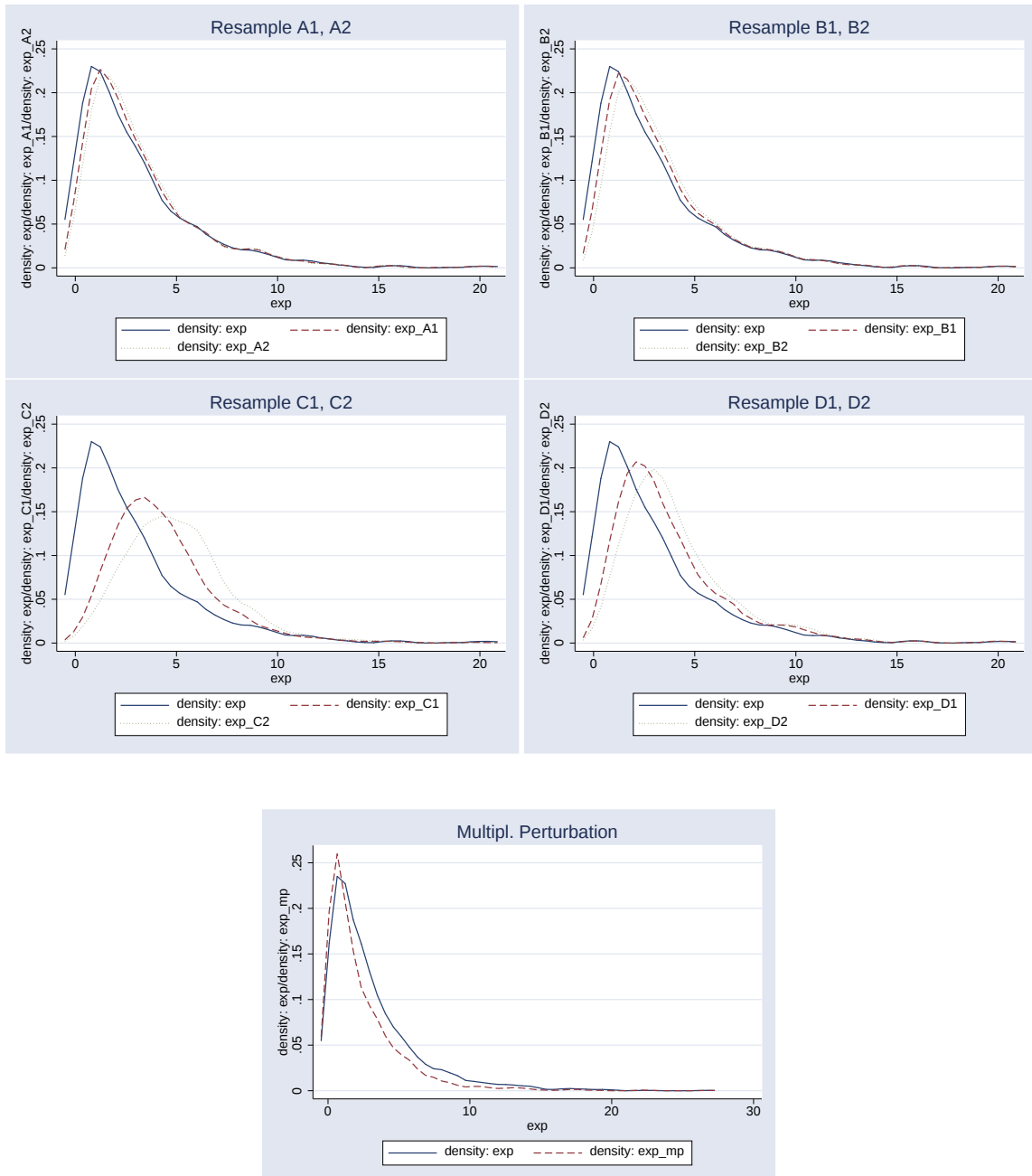
Figure 2: Exponential Distribution
