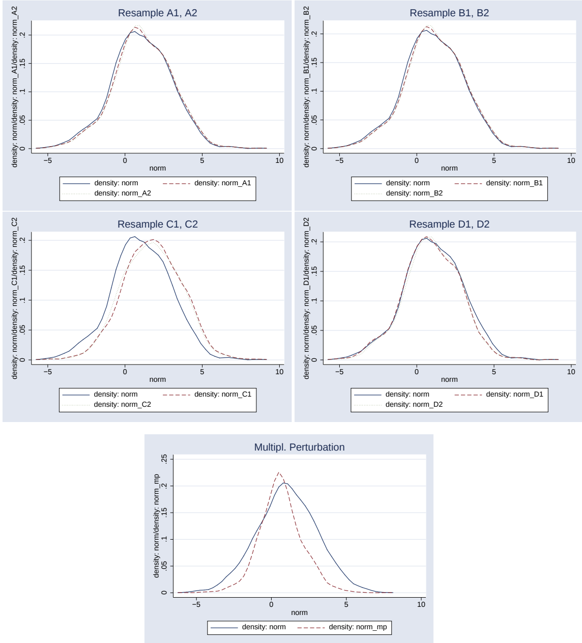
Figure 1: Normal Distribution
