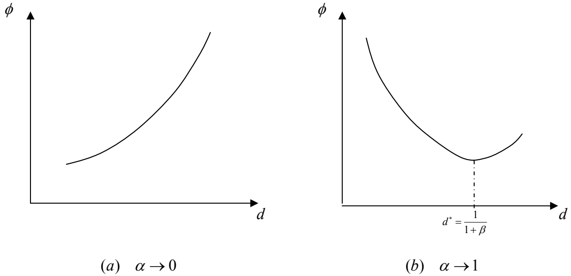
Figure 3: The pure demand-side effect of d on \phi
