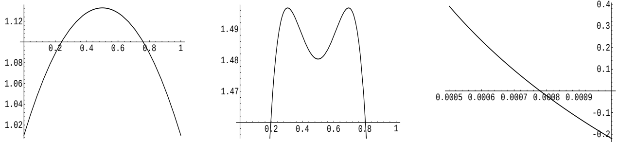
Figure 4.1: The function \psi defined in (4.1) in the case \lambda = 0.1 (left panel) and \lambda = 0.001 (middle panel). In the case \lambda = 0.1 the maximum is attained at the point d = 1/2 and the exact D -optimal design for the linear regression model (3.1) with correlation structure (2.2) and n = 3 observations is equally spaced at 0, 1/2 and 1. If \lambda = 0.0001 there are two maxima of \psi corresponding to the two exact D -optimal designs \{0, 0.2459, 1\} and \{0, 0.7541, 1\} . The right panel shows the second derivative of the function \psi at d = 1/2 for some small \lambda .
