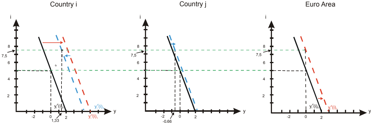
Figure 5: Idiosyncratic Demand Shock in Country i: \varepsilon_{i,1} = 3
