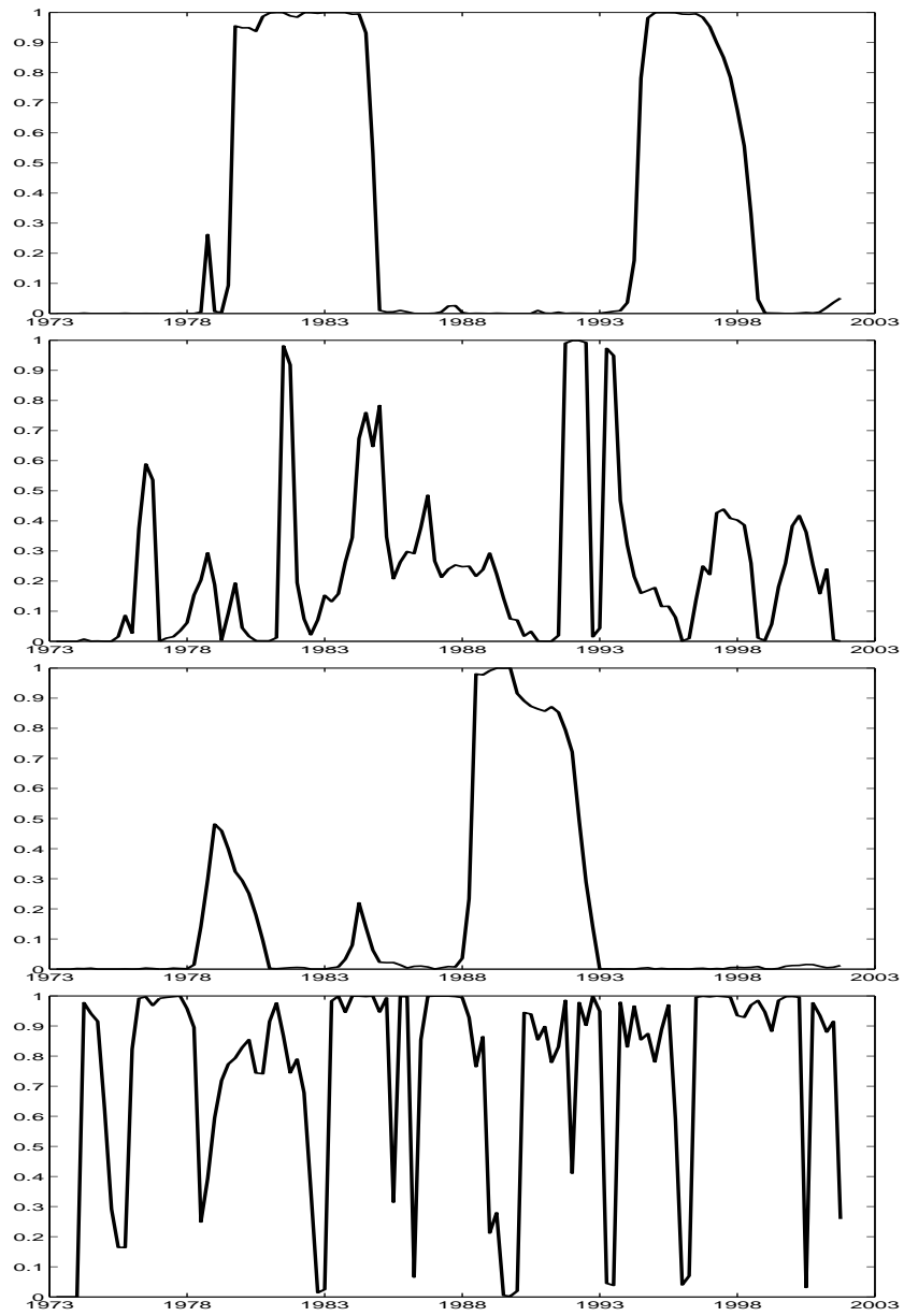
Fig. 6. Smoothed probabilities of state 1 of the Markov-Switching model of the Taylor rule according the model in Equation 12: USA (top panel), UK (second panel), Germany (third panel), France (bottom panel)
