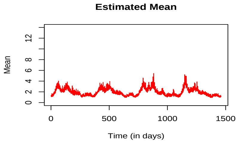
Figure 1: Astma series (top left) its autocorrelation function (top right) the series \hat{\mu}_t for an Poisson-GLARMA model (bottom left) and the autocorrelation function of the estimated Pearson residuals (bottom right).
