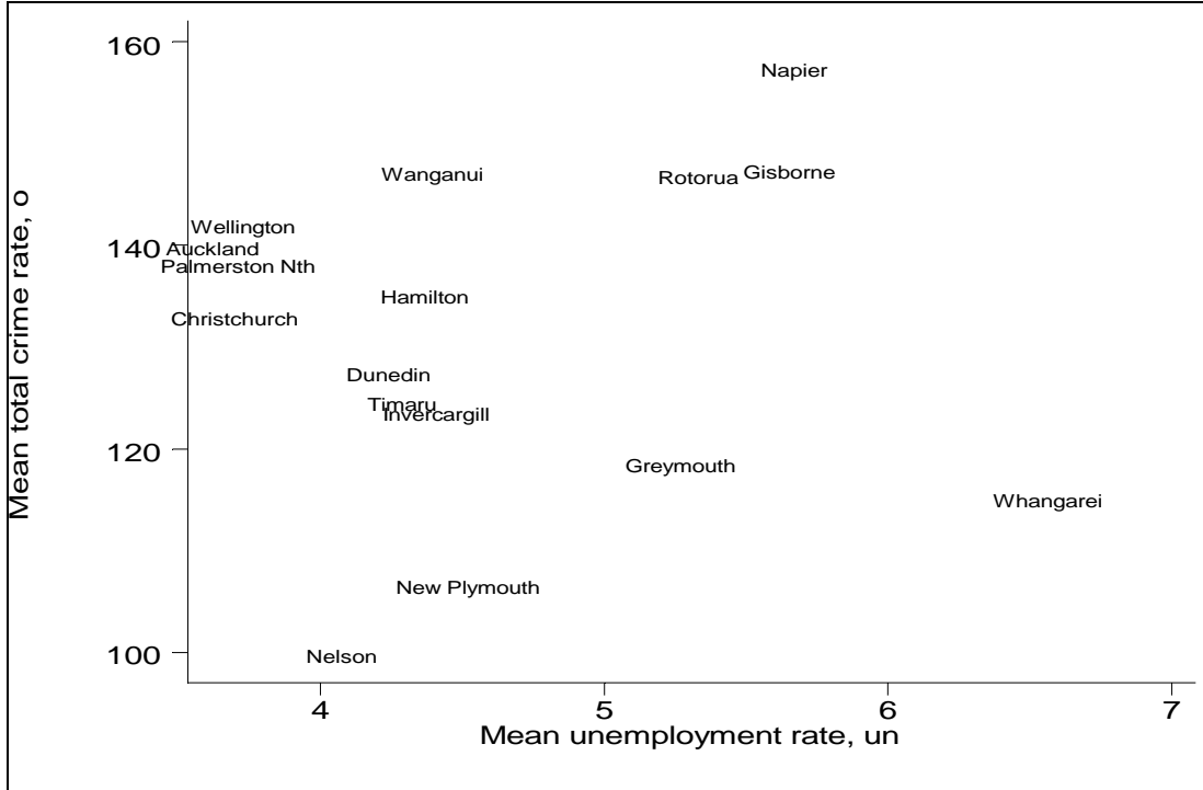
Scatter Plot of Time-Averaged Crime and Unemployment Rates
