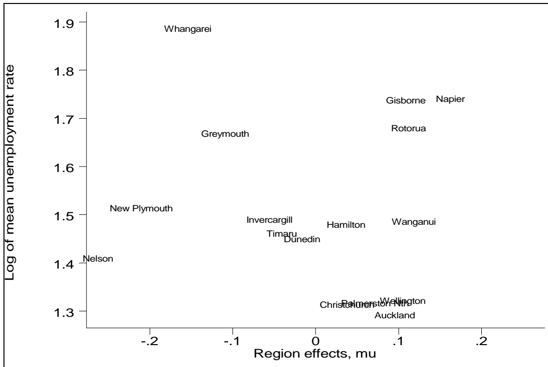
Scatter Plot of Time-Averaged Unemployment Rate and Estimated Region Effects
