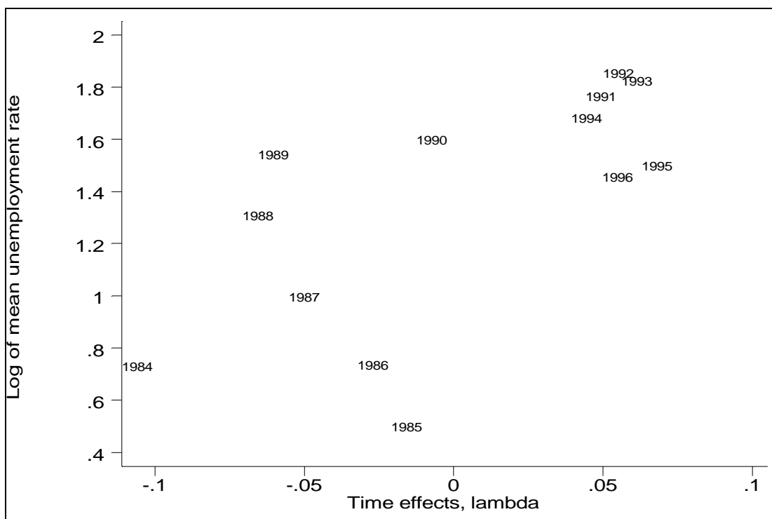
Scatter Plot of Region-Averaged Unemployment Rate and Estimated Time Effects
