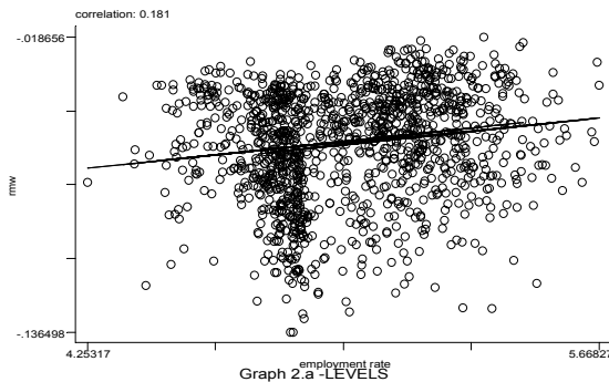
Graph 2.a - LEVELS
