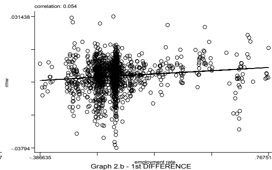
Graph 2.b - 1st DIFFERENCE
