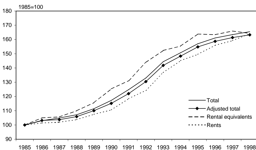
Figure 4: Fisher indices for housing
