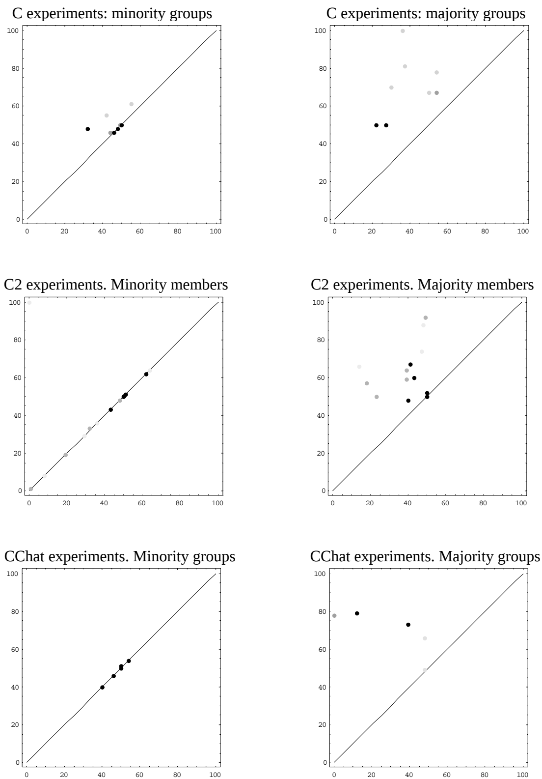
FIGURE 5 Group Behavior - Group Cutpoints
