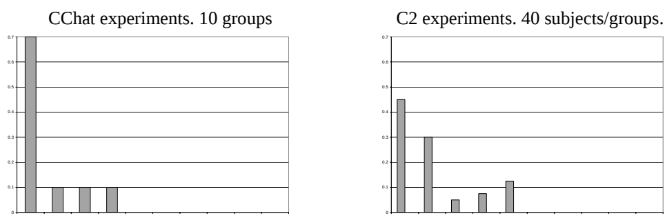
Figure 4b: Average errors' distance relative to random voting
