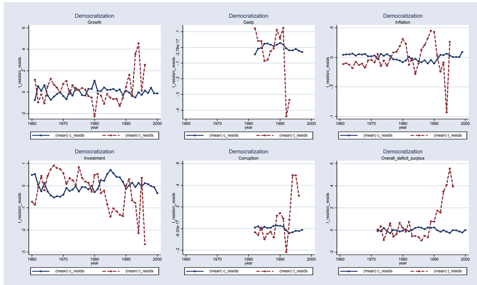
Figure 2 Estimated residuals for controls (always) and treated (before democracy)
