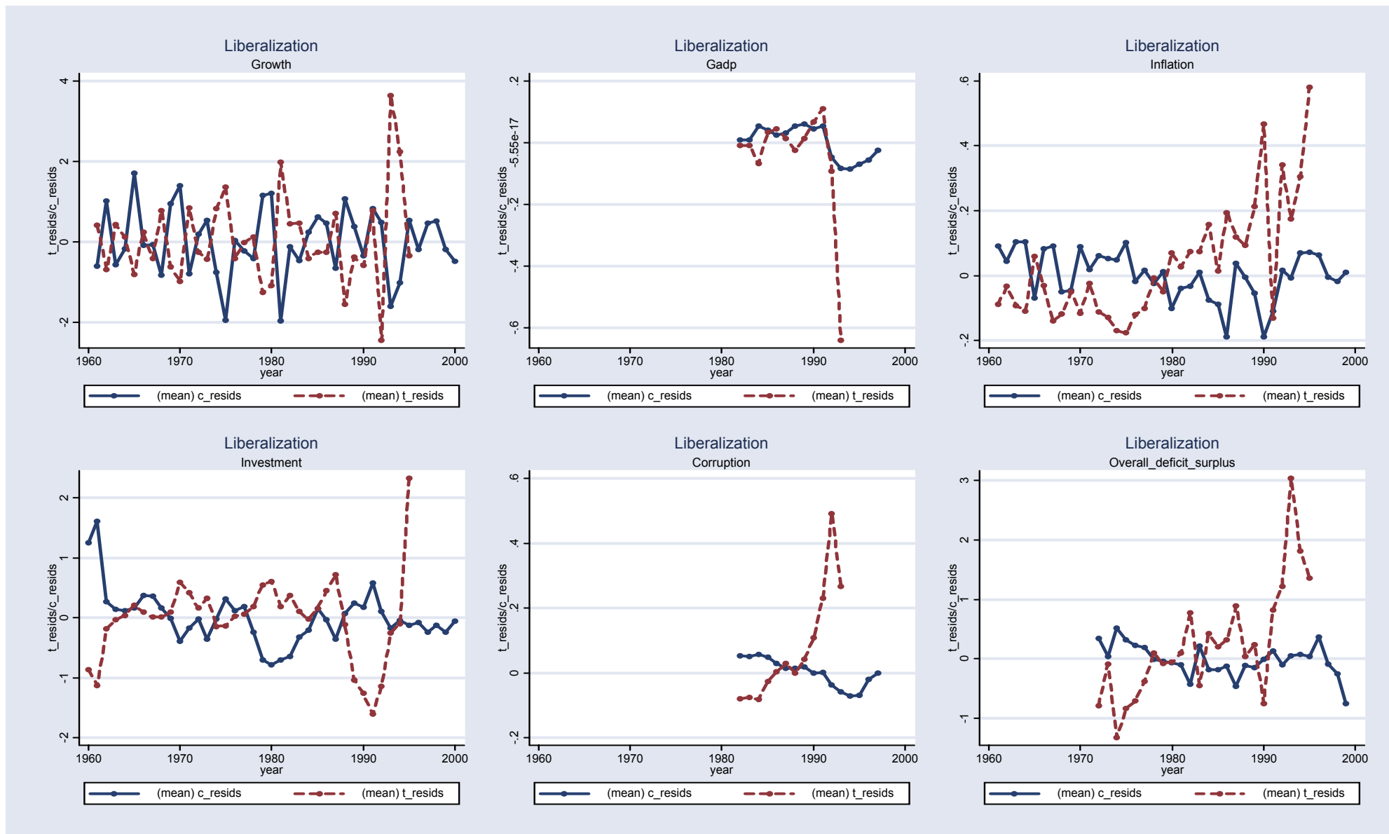
Figure 1 Estimated residuals for controls (always) and treated (before liberalization)
