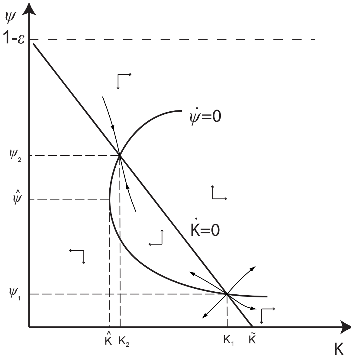
FIGURE 5 \theta < 1, \delta < 0
