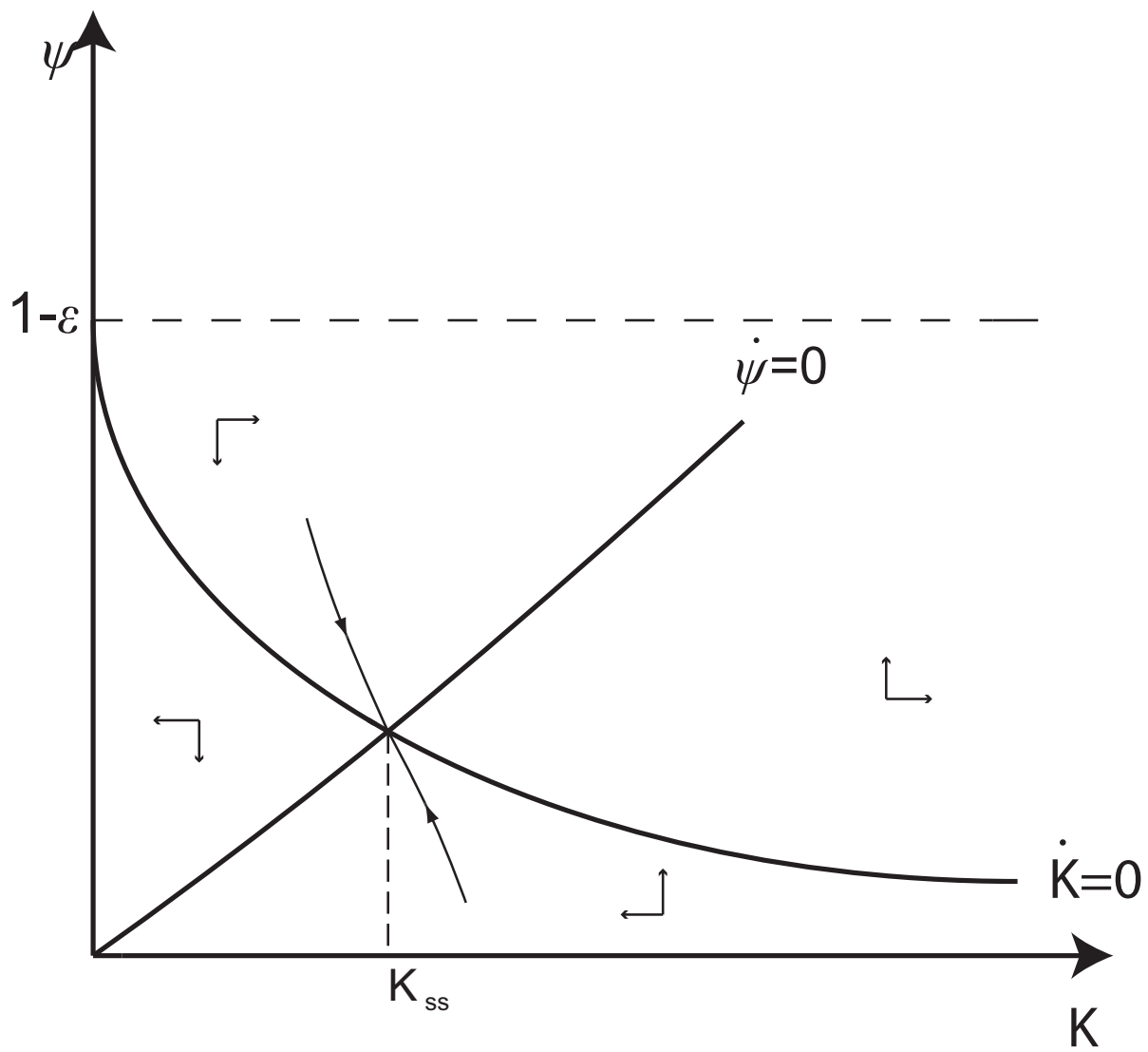
FIGURE 4 \theta=1, \delta>0
