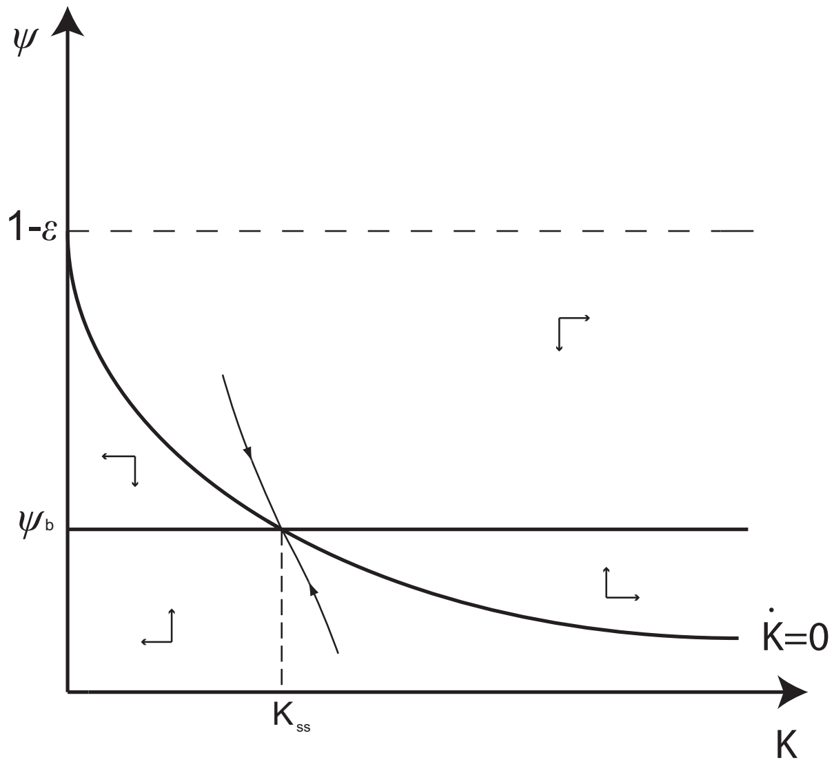
FIGURE 1 \theta=1, \delta=0
