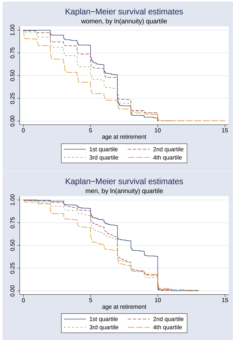
Figure 4: Kaplan-Meier estimator without censoring for the period 2000-2003 by income quartiles for women (upper panel) and men (lower panel). The numbers on the horizontal axis denote the years after age 55.
