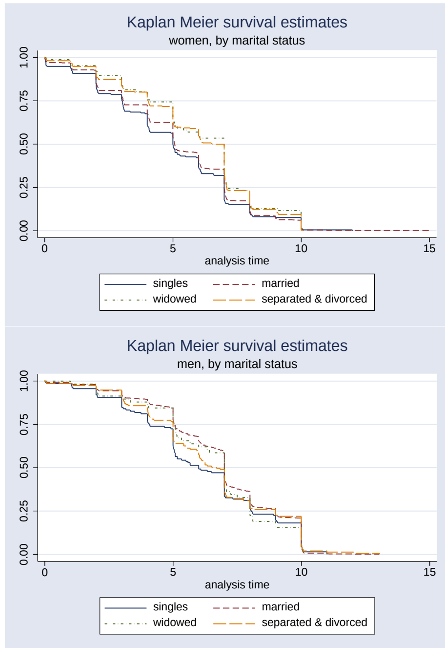
Figure 3: Kaplan-Meier estimator without censoring for the period 2000-2003 by marital status for women (upper panel) and men (lower panel). The numbers on the horizontal axis denote the years after age 55.
