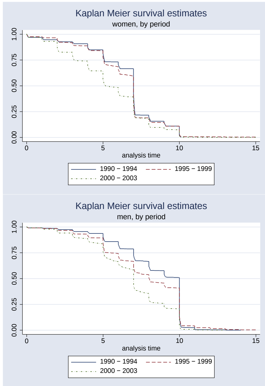
Figure 2: Kaplan-Meier estimator without censoring by period for women (upper panel) and men (lower panel). The numbers on the horizontal axis denote the years after age 55.
