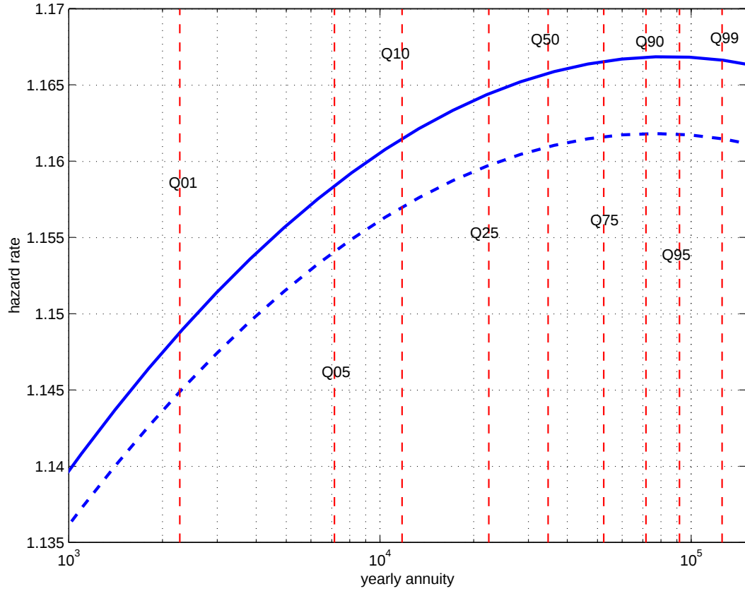
Figure 6: Relative hazard rates for estimations II(m) (= dashed line) and IV(m) (= solid line) (with time trend) as a function of yearly deflated annuity (base = annuity of 1 SFR). ‘ Q_x ’ denotes the x th quantile of the annuity distribution for men.
