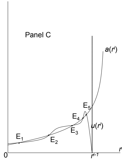
Figure 2. Equilibria
