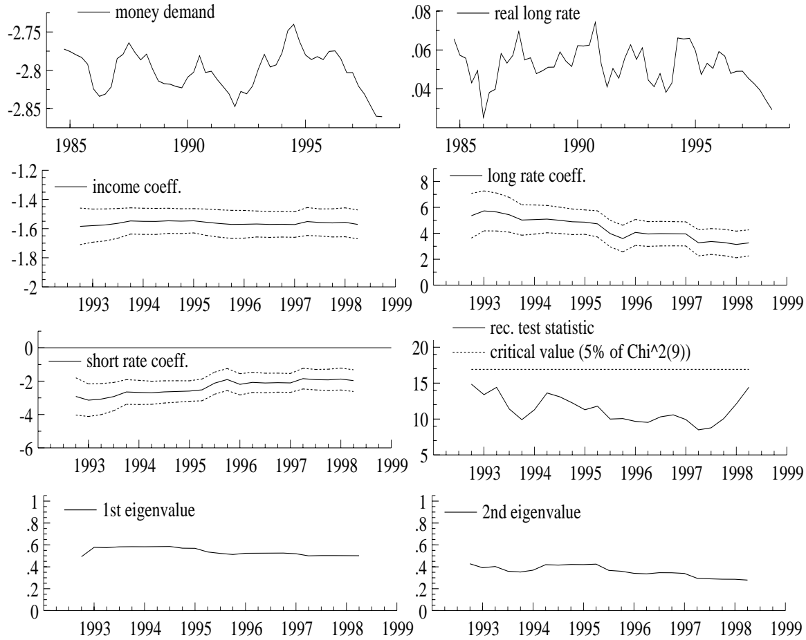
Cointegration relationships; recursively estimated coefficients together with two standard error bands on income, long and short term interest rates; recursive test of restrictions; recursive eigenvalues
