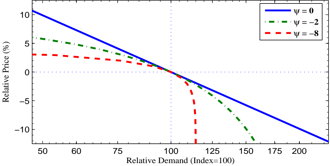
Figure 1: Quasi-Kinked Demand
