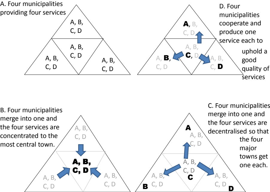
Figure 2: Theoretical illustration of merging effects
