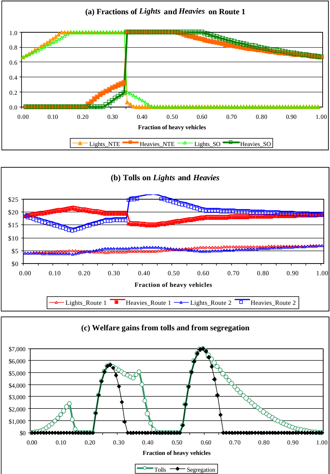
Figure 2: Results for Variant 6: l_H^L = 2 , v^H = \$25/hr
