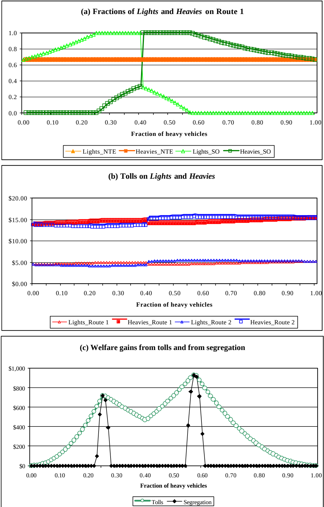
Figure 1: Results for Variant 2: v^H = \$15/hr
