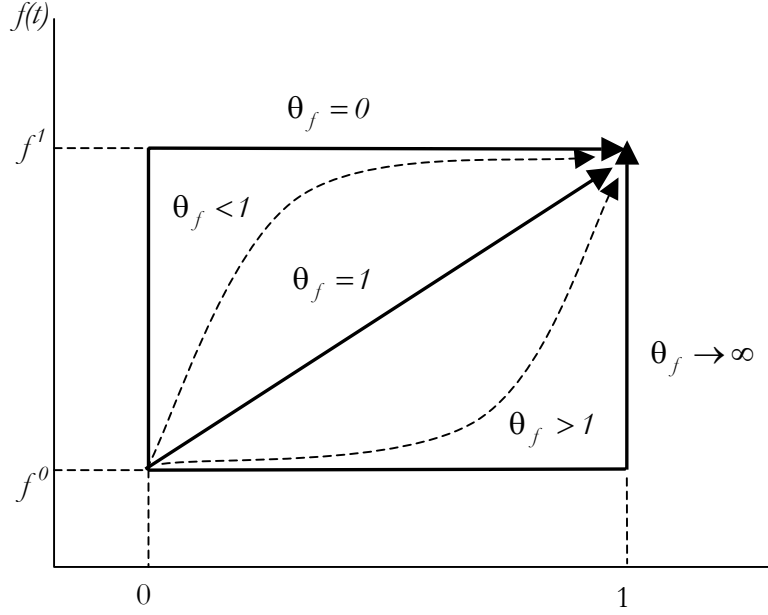
Figure 1. Several temporal paths for factor f
