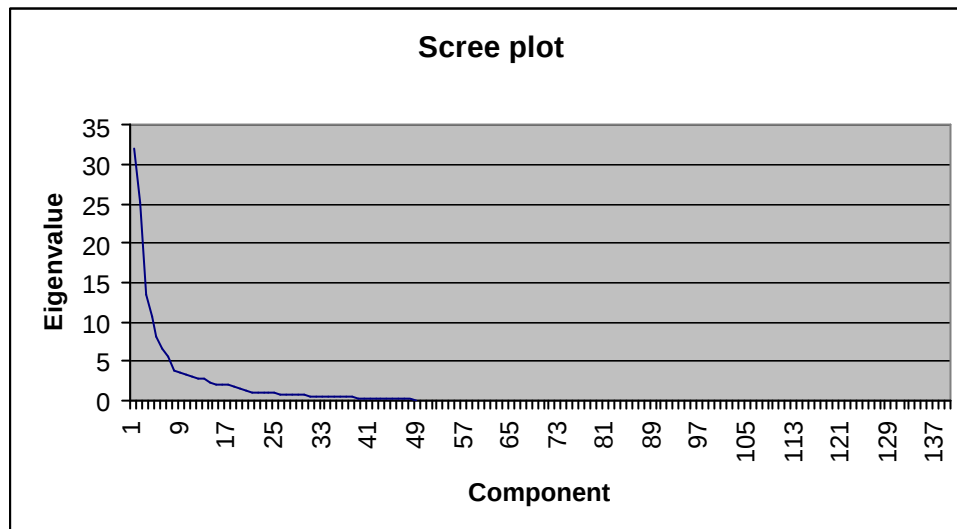
Figure 1: Plot of Eigenvalues (Scree Plot)
