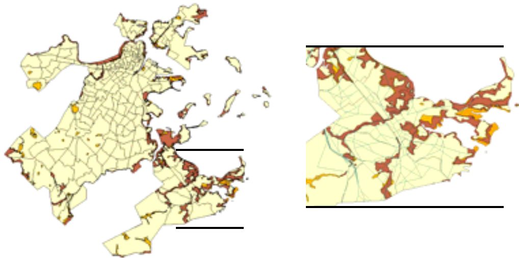
Figure 7. Overlay of Flood Plains and Transportation Network in one of Seven CLIMB Sub-regions.
