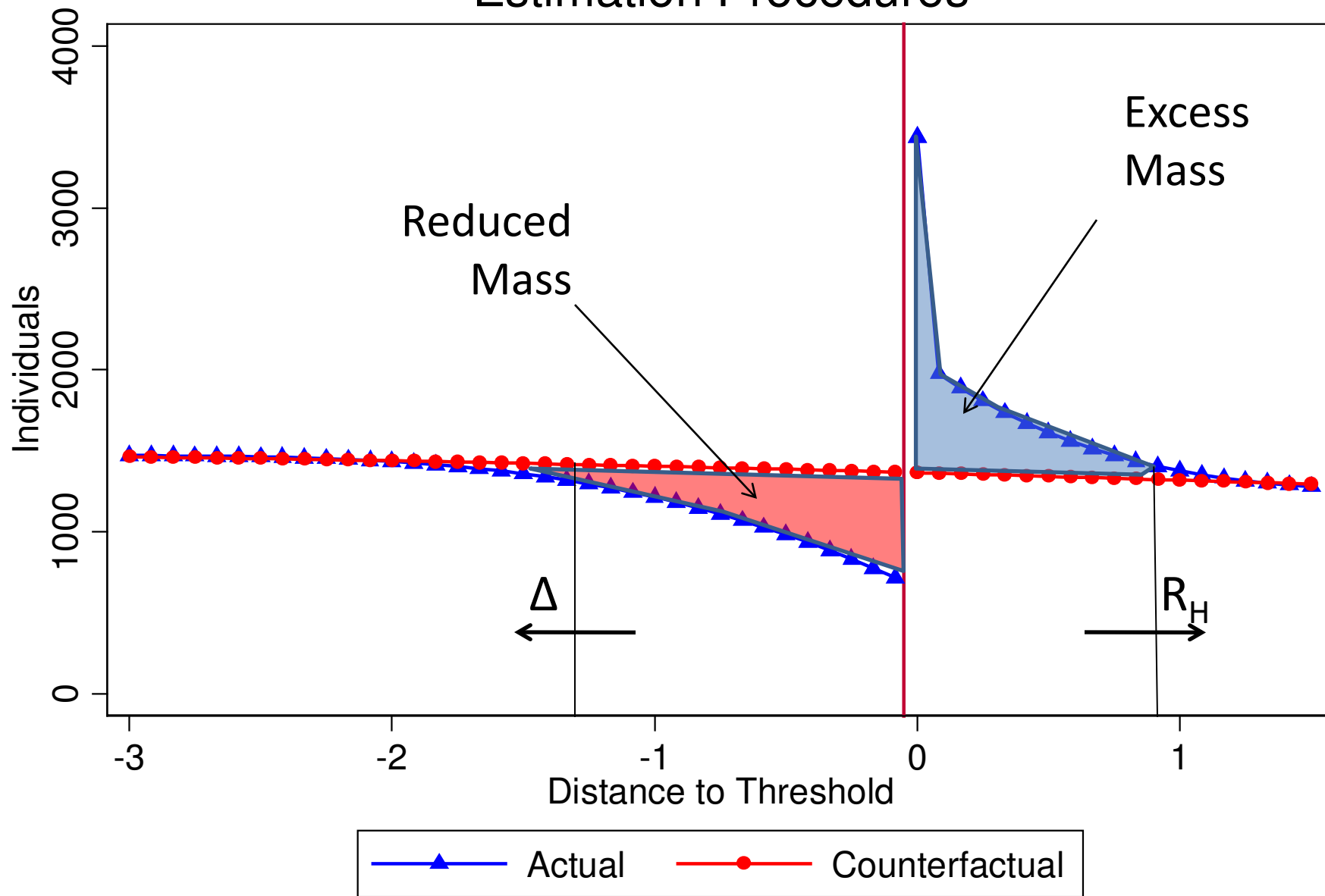
Fig. 15. Estimation Procedures
