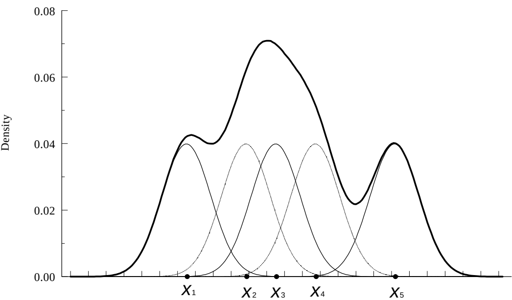
GRAPH 2. Density Estimation
