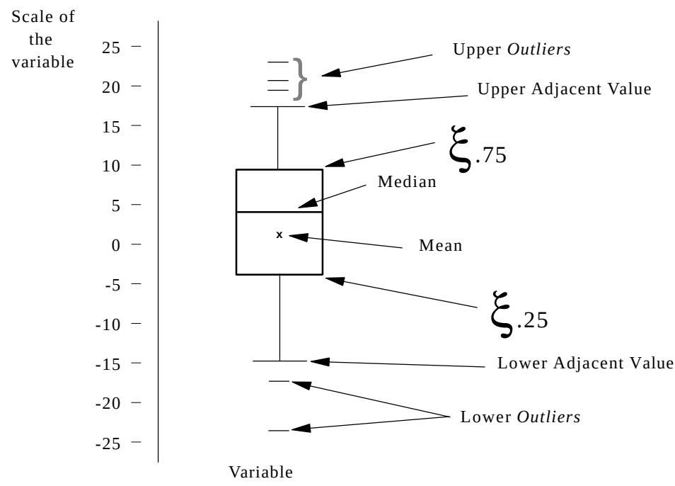
GRAPH 1. Box-Plot
