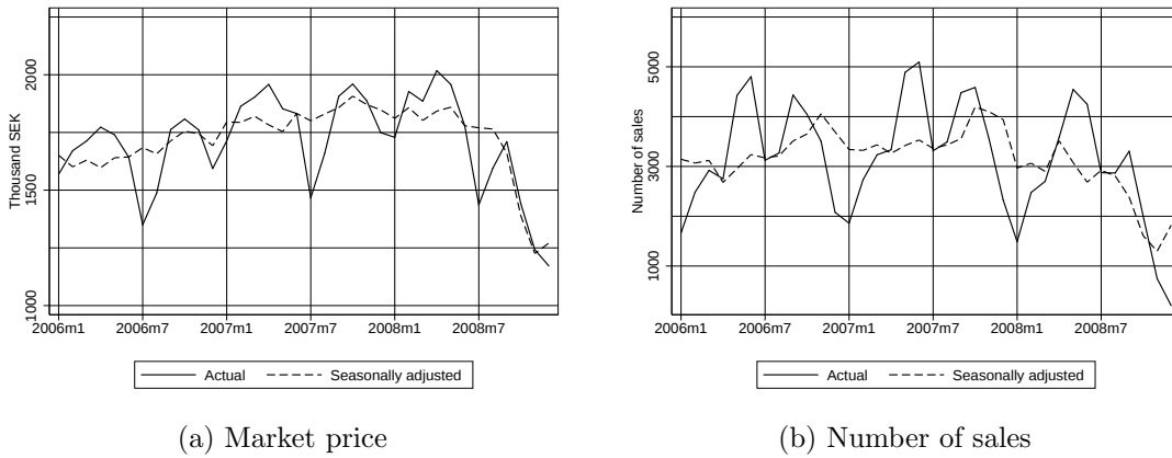
Figure 4: Time series
