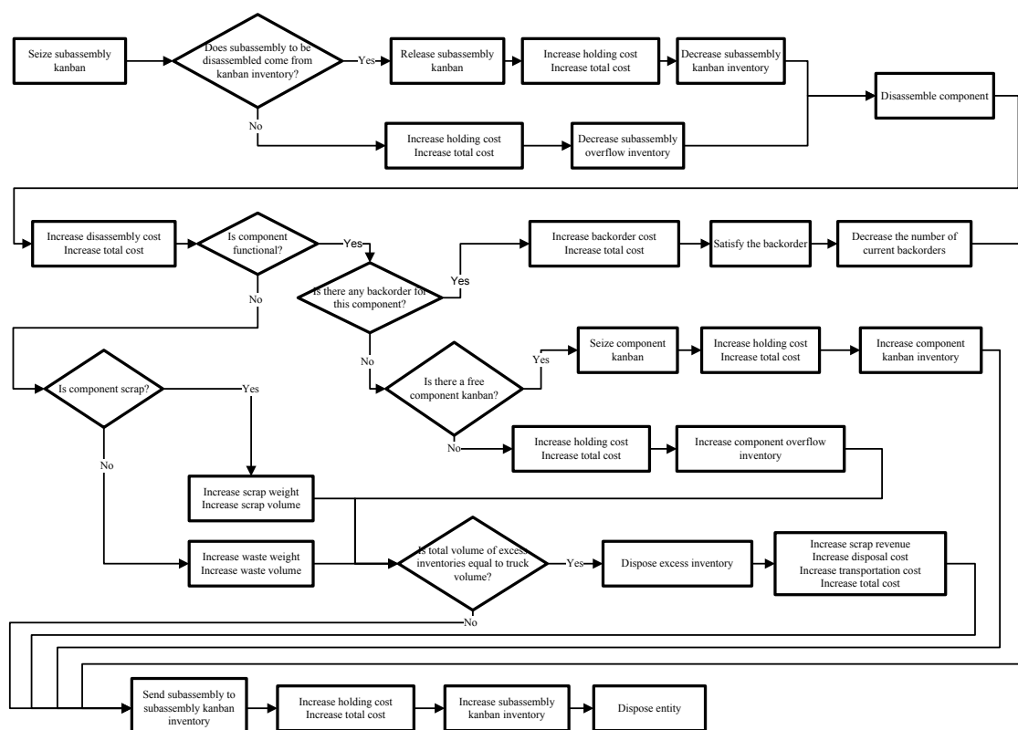
Figure 11 Disassembly operations authorized by a subassembly kanban for the case of SEPs.
