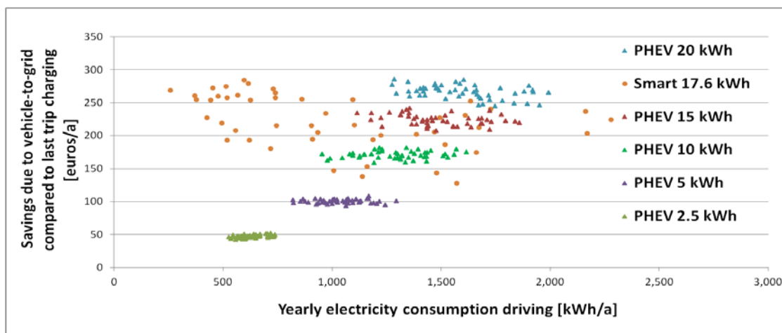
Figure 14: Vehicle-to-grid savings compared to uncontrolled charging
