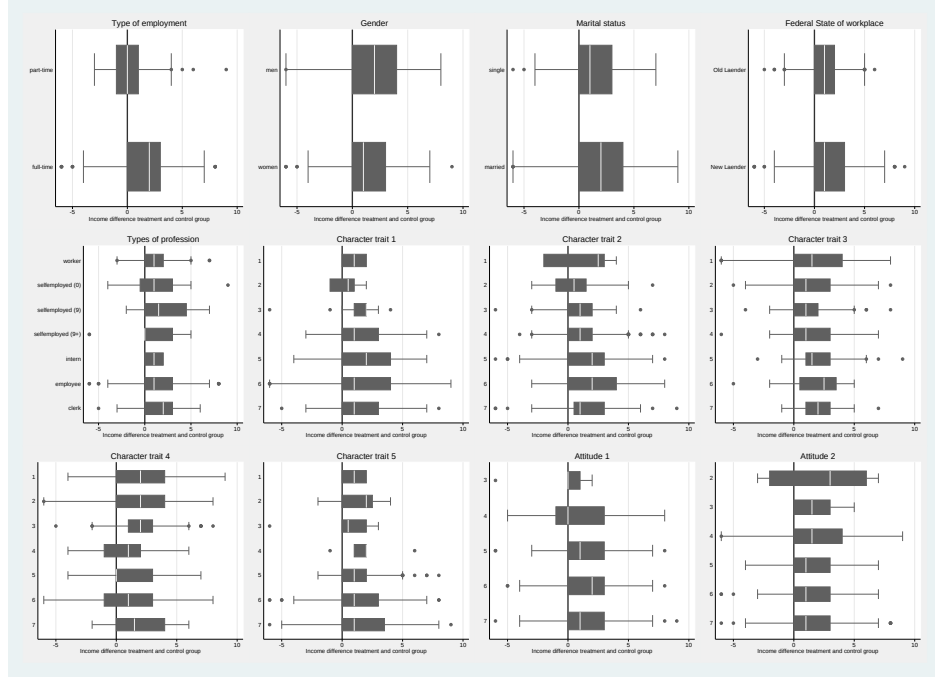
Figure 1: Box plot charts of the matching variables
