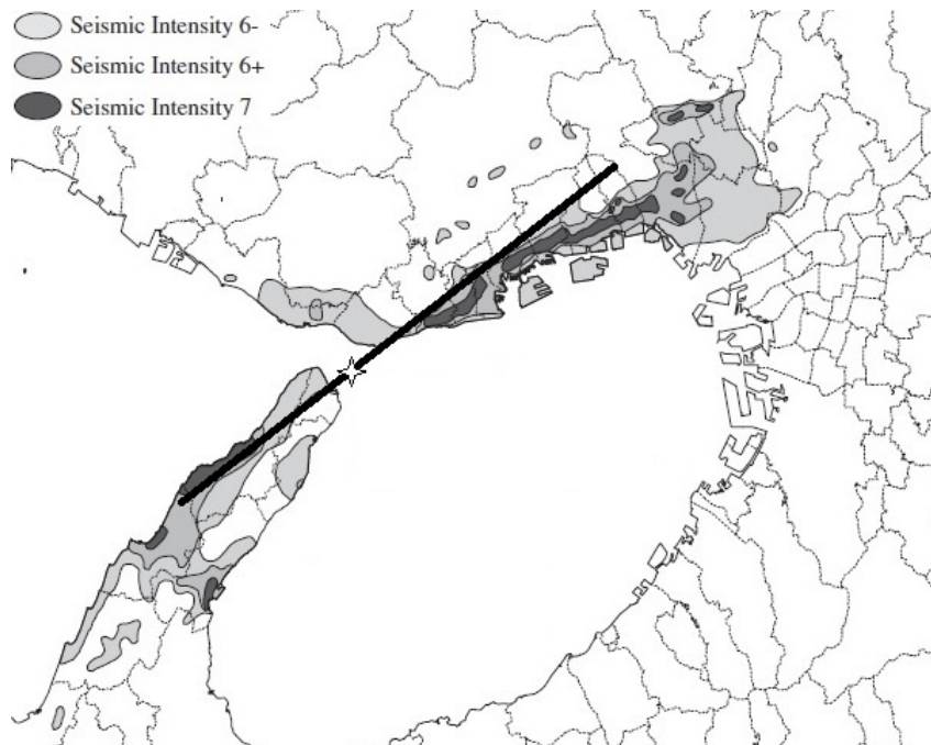
Figure 3: Seismic intensity
