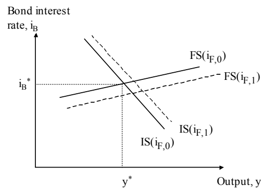
Figure 4. The effect of a lower policy rate in normal times (i_{F,0} > i_{F,1}) .
