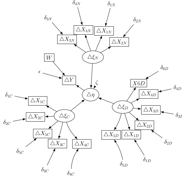
Figure 1: Path Diagram of the Idealized Structural Equation Model
