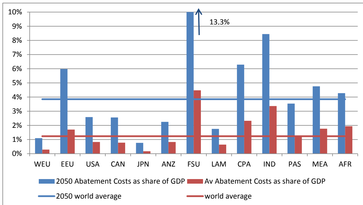
Figure 4: Approximated abatement costs ( 0.5 \cdot (\text{BAU emissions} - \text{actual emissions}) \cdot \text{carbon price} ) in the [tax] scenario as share of GDP in [BAU] for 2050 and the average abatement costs from 2012 to 2050.
