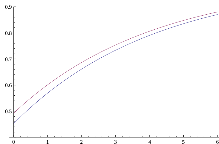
Figure 1. Survival probabilities, \phi_1(u) and \phi_2(u) .
