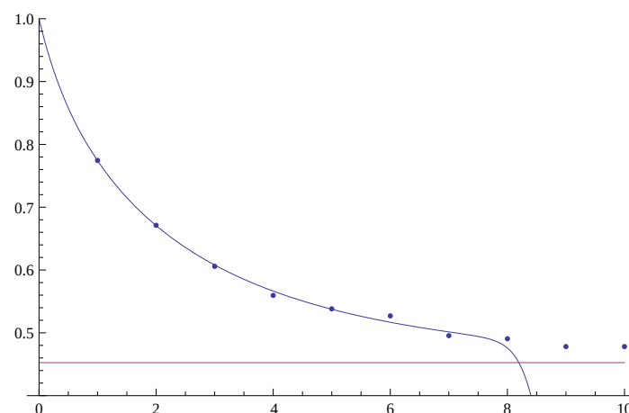
Figure 2. The probability of reaching level x before ruin for J(0) = 1, X(0) = 0 .
