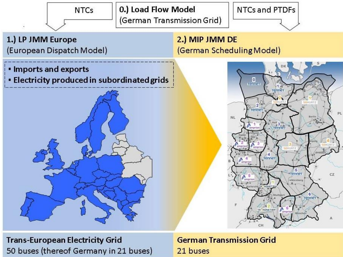
Figure 1: Model framework and geographical scope
