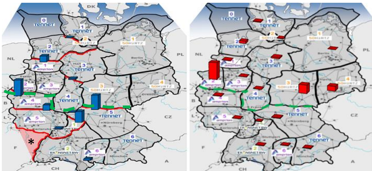
Figure 2: Congestion amount for the top 10 regional borders (left) and negative redispatch amount by region (right) for Germany (reference scenario 2015)
